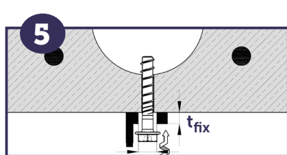
5. Install the screw anchor very gently by screwdriver or torque wrench. Avoid overtightening.
