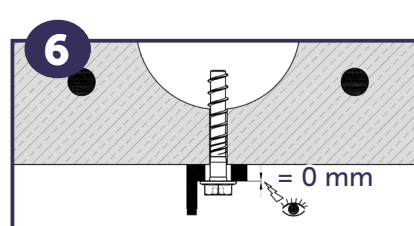
6. Ensure that the screw anchor head fully rests without any gap on the fixture and is not damaged
